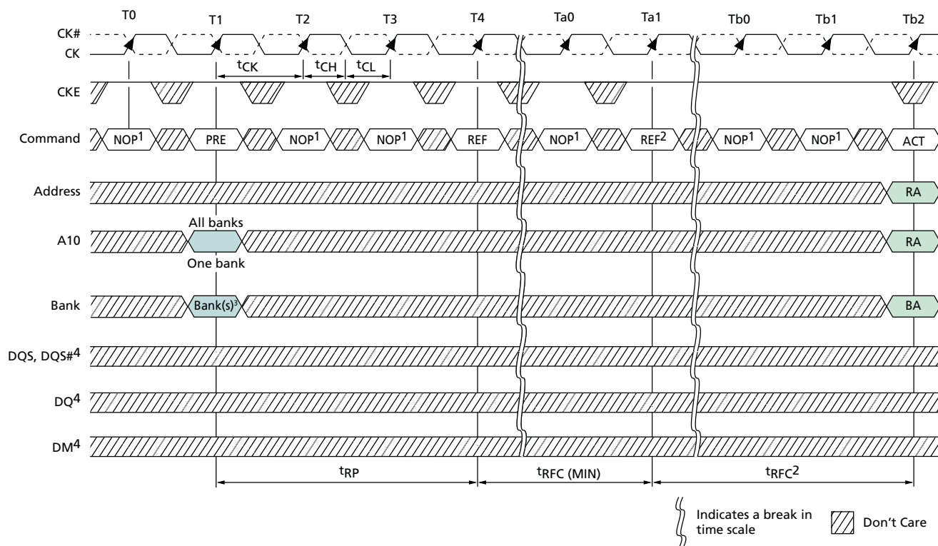
Figure 67: Refresh Mode
