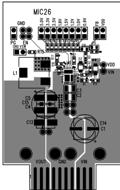
MIC26903-ZA Evaluation Board Top Layer
