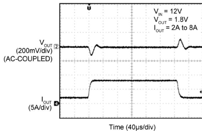
Transient Response
