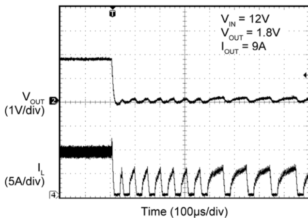
Short Circuit
