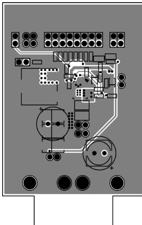
MIC26903-ZA Evaluation Board Mid-Layer 2
