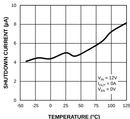
V_{IN} Shutdown Current vs. Temperature
