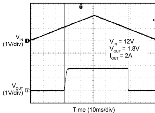
Enable Thresholds
