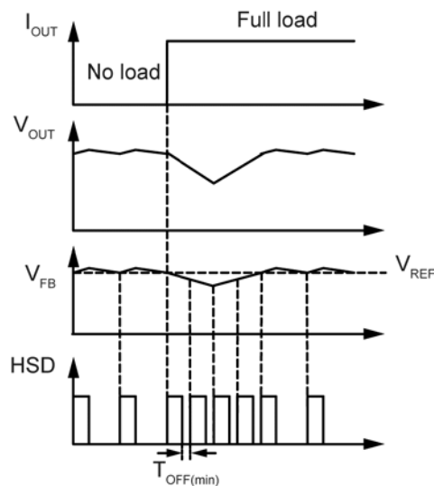
Figure 2. MIC26903-ZA Load Transient Response
