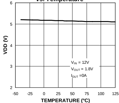
V_{DD} vs. Temperature
