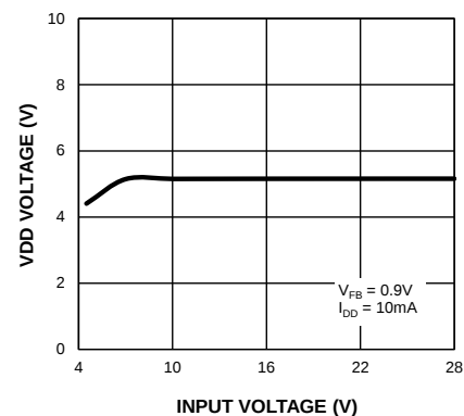
V_{DD} Output Voltage vs. Input Voltage
