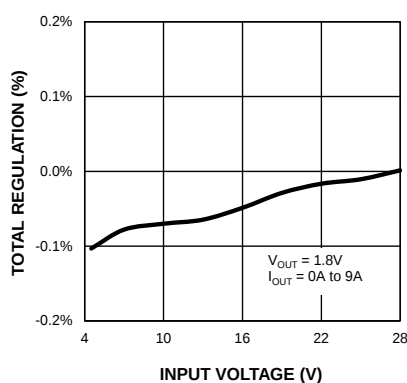
Total Regulation vs. Input Voltage
