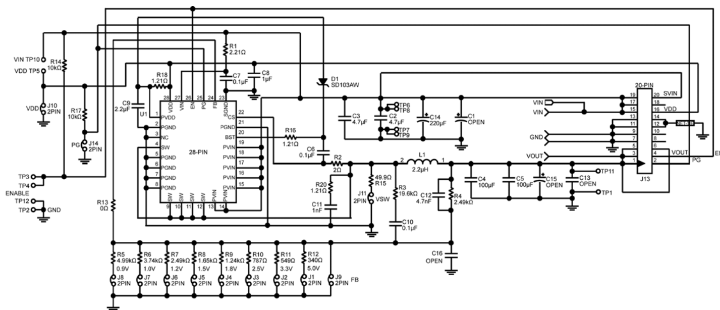
Schematic of MIC26903-ZA Evaluation Board (J11, R13, R15 are for testing purposes)
