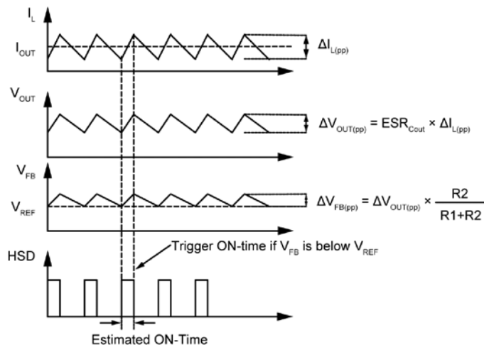
Figure 1. MIC26903-ZA Control Loop Timing
