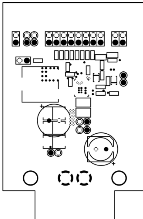
MIC26903-ZA Evaluation Board Mid-Layer 1 (Ground Plane)
