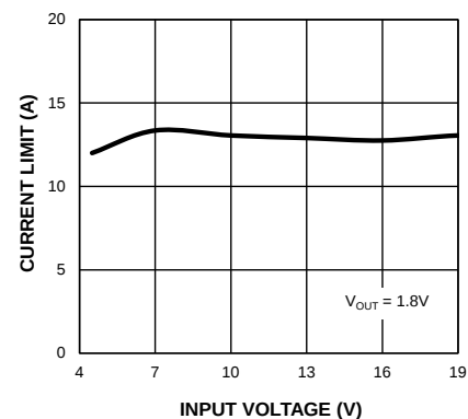
Output Current Limit vs. Input Voltage
