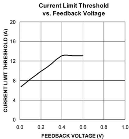
Figure 3. MIC26903-ZA Current-Limit Foldback Characteristic
