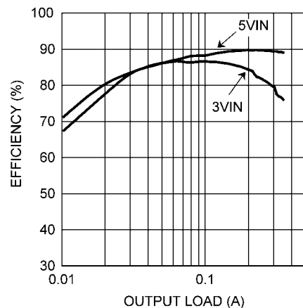
Efficiency vs Load Current V_O = 12V
