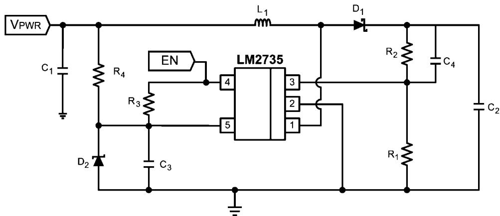
LM2735X (1.6MHz): V PWR = 9V, V out = 12V @ 500mA
