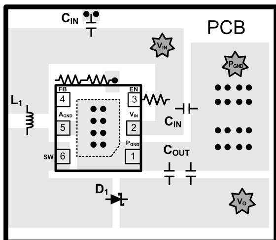
Example of Proper PCB Layout
