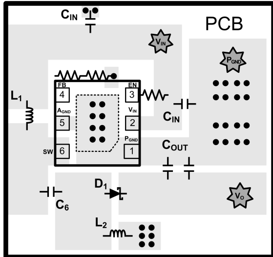
FIGURE 17. SEPIC PCB Layout
