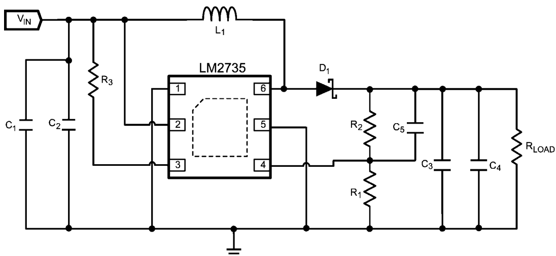
LM2735Y (520kHz): V_{in} = 3.3V , V_{out} = 20V @ 150mA
