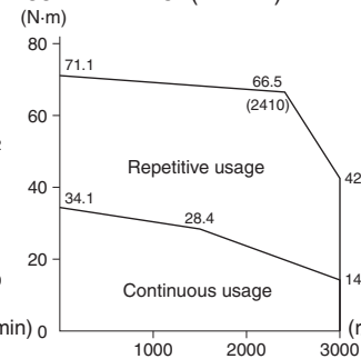
R88M-W15K015T (15 kW)
