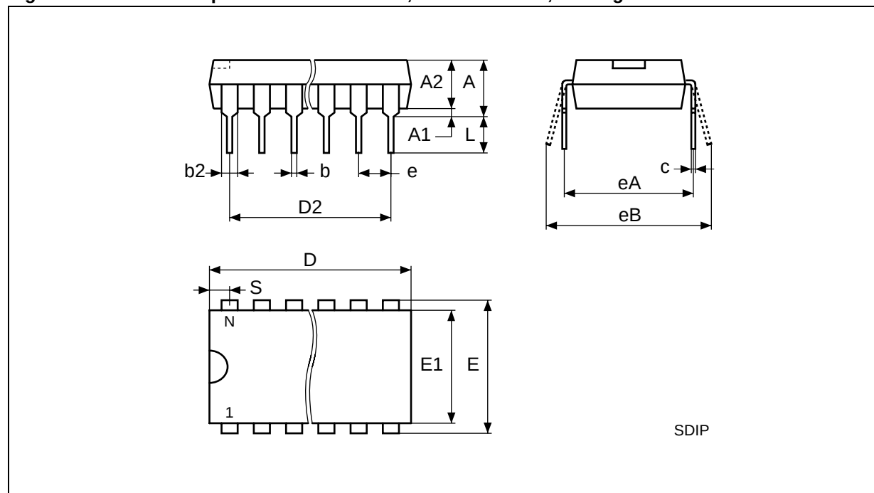
Figure 14. SDIP42 - 42 pin Shrink Plastic DIP, 600 mils width, Package Outline
