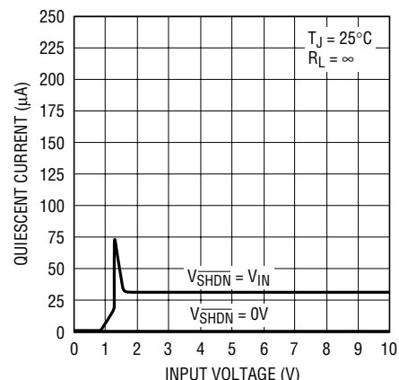
LT1763-1.5 Quiescent Current
