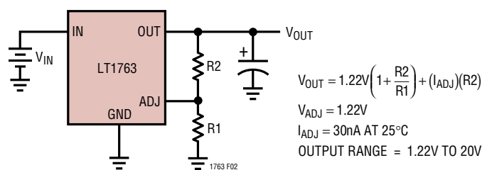
Figure 2. Adjustable Operation
