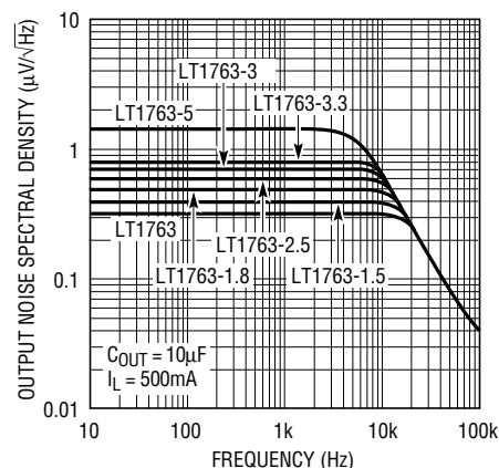
Output Noise Spectral Density CBYP = 0
