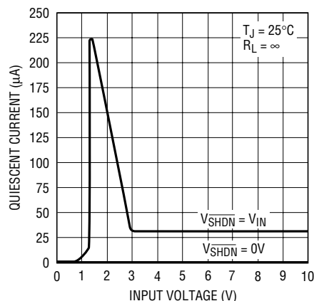
LT1763-3 Quiescent Current
