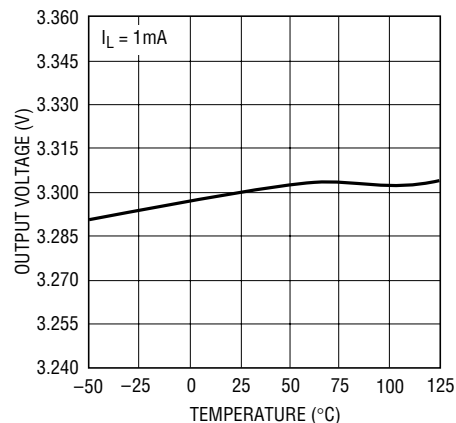
LT1763-3.3 Output Voltage
