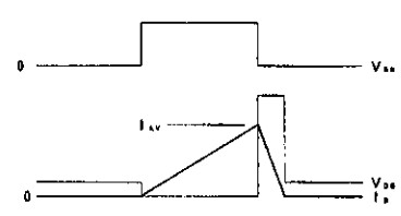
図2 動作波形 Operating waveforms
