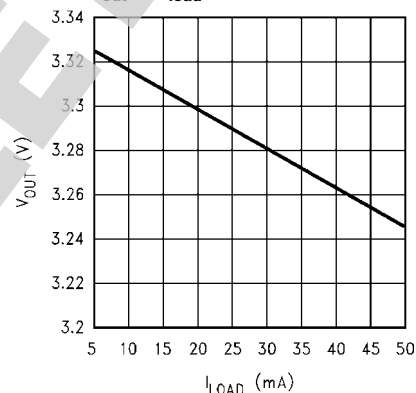
V_{out} vs I_{load} (Step-Down)
