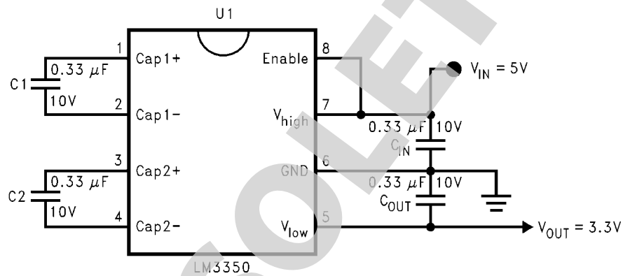
FIGURE 3. Step-Down Converter
