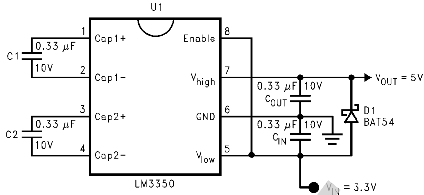
FIGURE 2. Step-Up Converter
