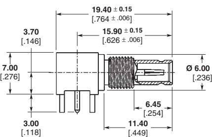
Part Number 1460060-1
