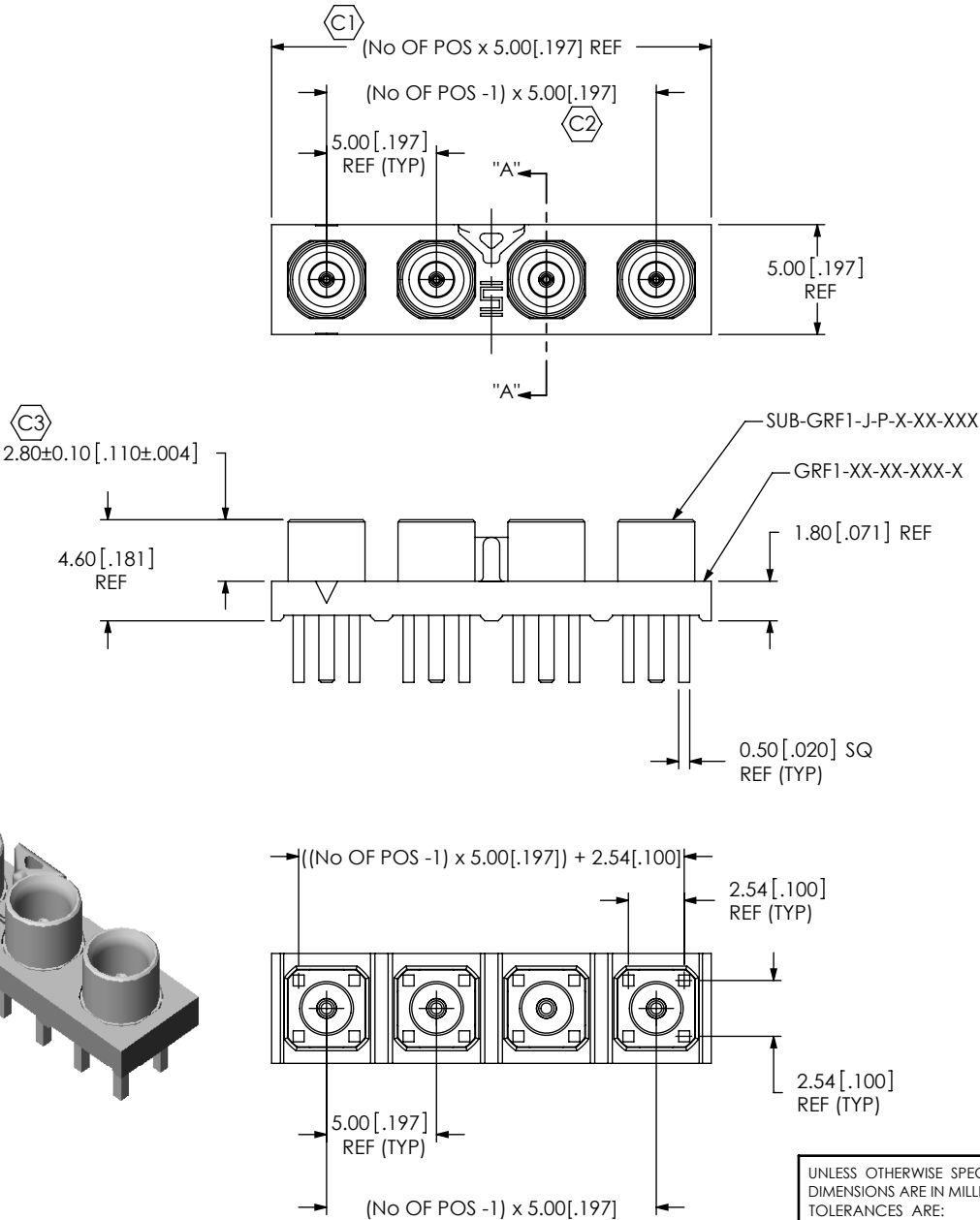
FIG. 1 GRF1-J-P-04-E-ST-TH1 SHOWN
