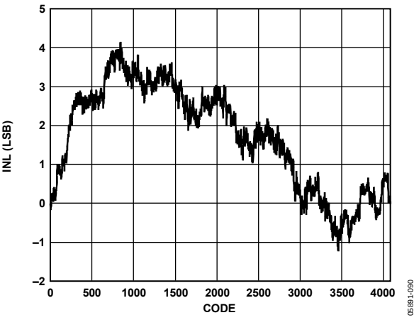
Figure 7. Typical Integral Nonlinearity (INL) Performance
