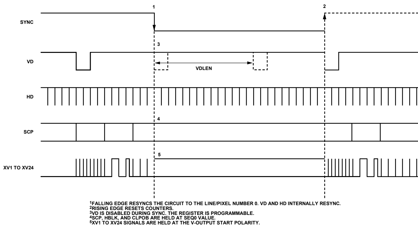
Figure 67. Enhanced SYNC Mode 2 with Vertical Signals Held at VTP Start Value
