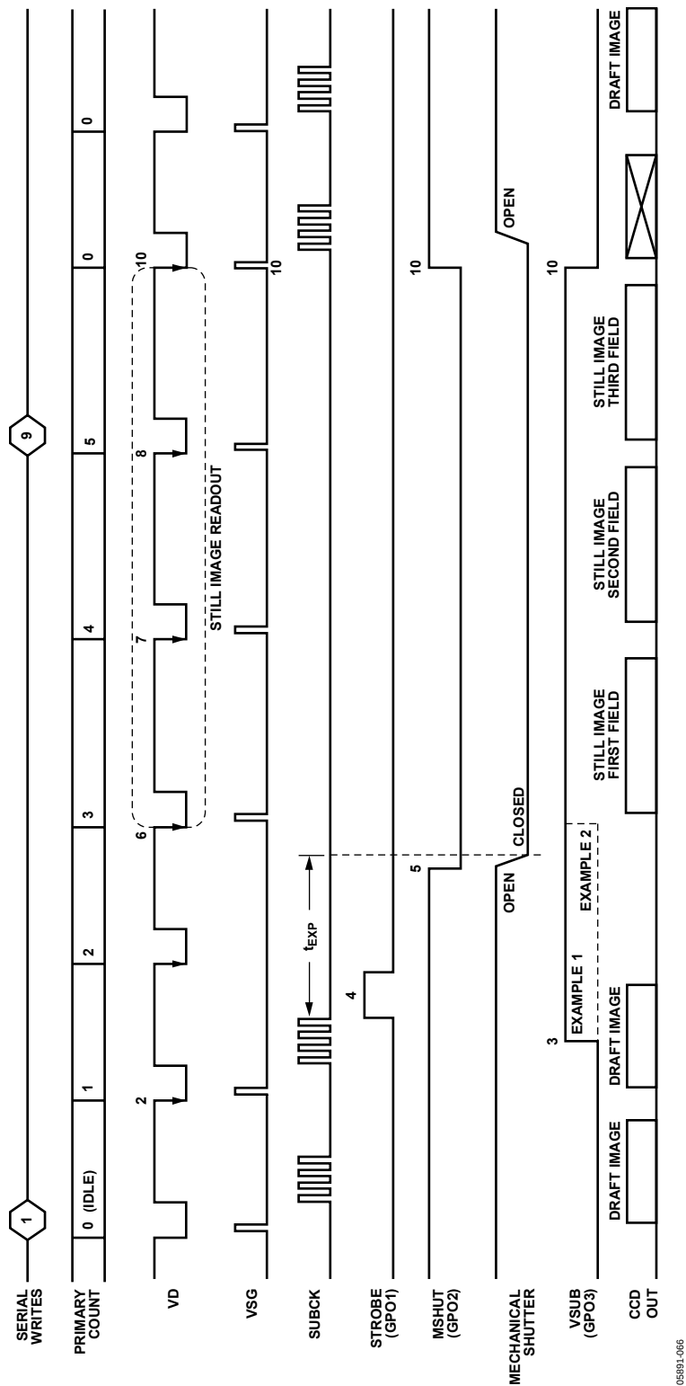
Figure 65. Complete Exposure/Readout Operation Using Primary Counter and GPO Signals
