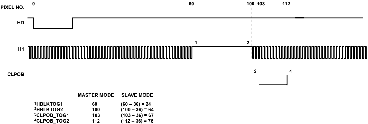
Figure 77. Example of Slave Mode Register Setting to Obtain Desired Toggle Positions
