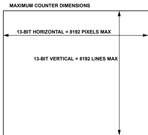
Figure 13. Vertical and Horizontal Counters
