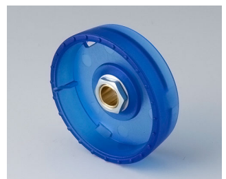
B8341066 STAR-KNOBS 41, with knurls PC (UL 94 HB) sapphire 41x14mm 6mm
