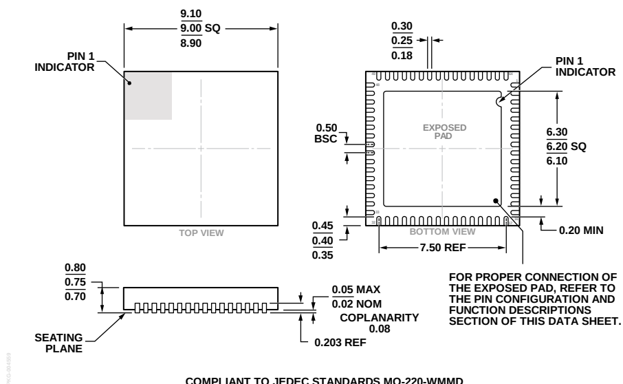
Figure 9. 64-Lead Lead Frame Chip Scale Package [LFCSP_WQ]
