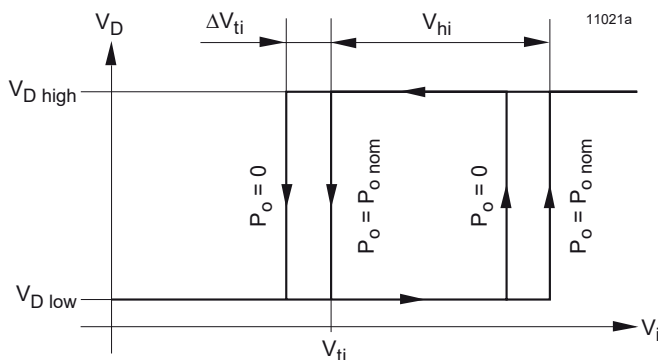
Fig. 38 Definition of V_{ti} , \Delta V_{ti} and V_{hi} (JFET output)
