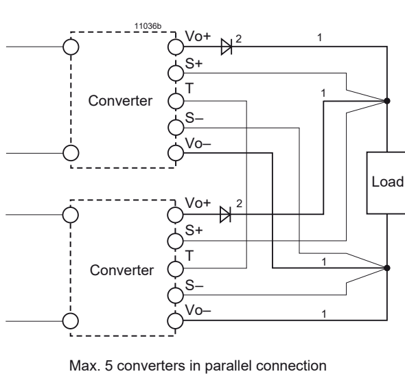
Max. 5 converters in parallel connection
