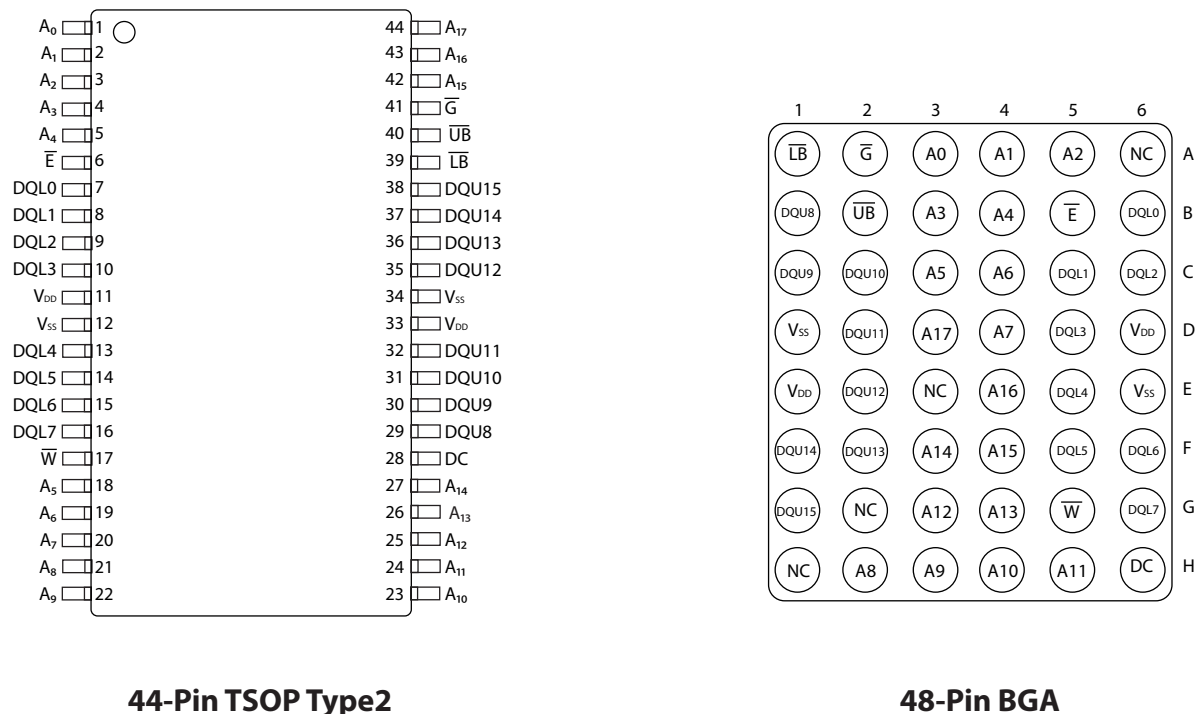
Figure 1.2 Pin Diagrams for Available Packages (Top View)
