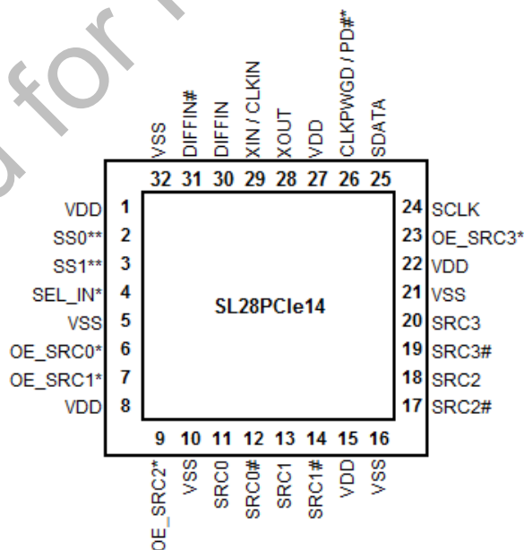
Pin Configuration
