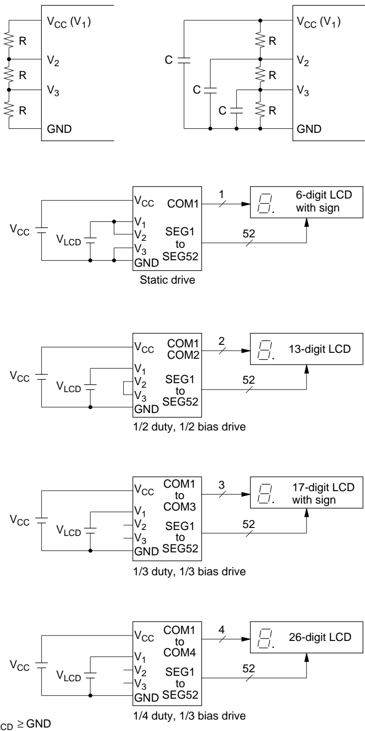
Figure 101 LCD Connection Examples
