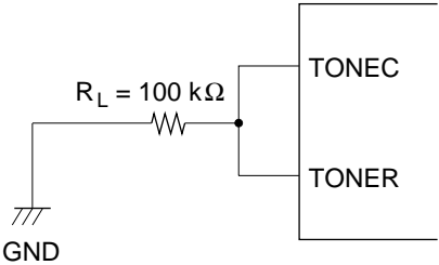
Figure 112 Distortion and dB CR Load Circuit
