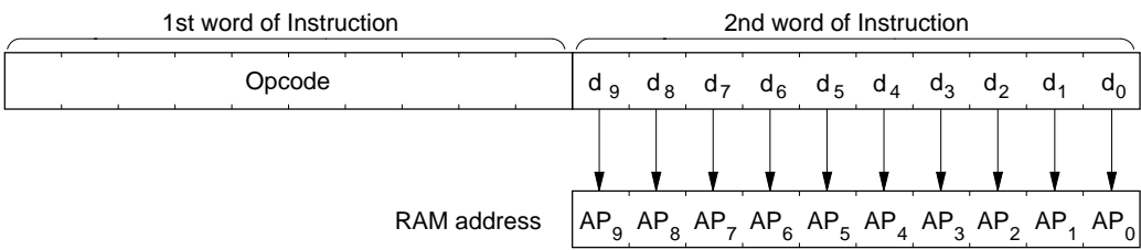
Direct Addressing
