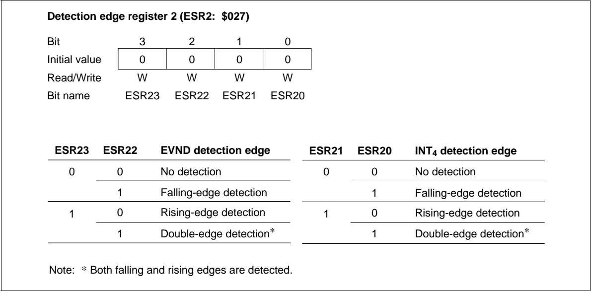
Figure 69 Detection Edge Select Register 2 (ESR2)
