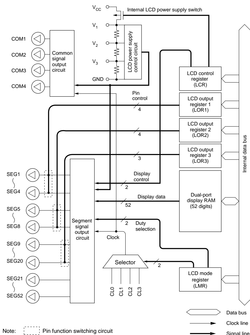
Figure 94 Block Diagram of Liquid Crystal Display Control System
