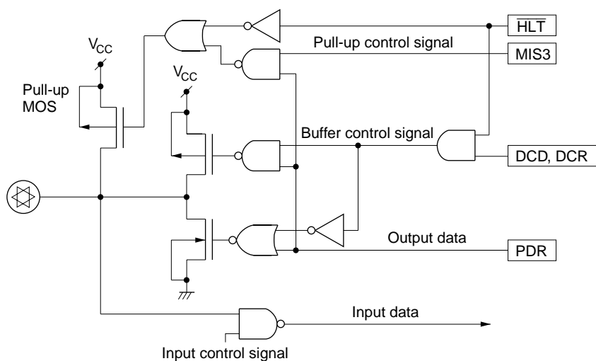
Figure 29 I/O Buffer Configuration
