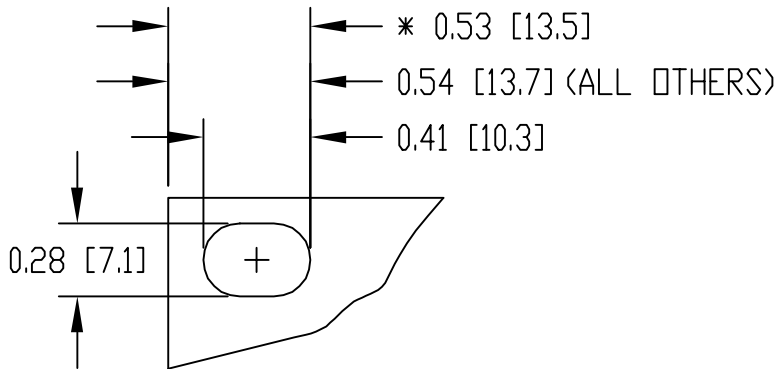
NOTCH DETAIL
