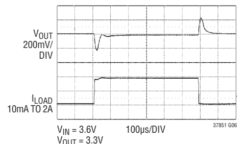
V_{OUT} Load Transient
