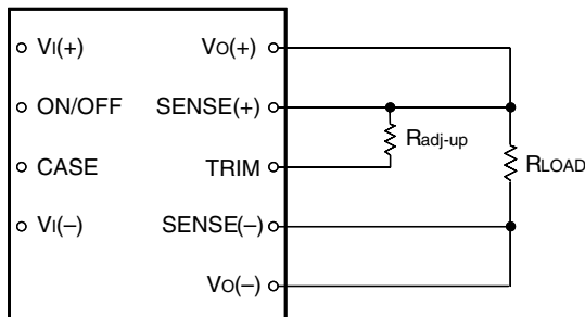
Figure 25. Circuit Configuration to Increase Output Voltage
