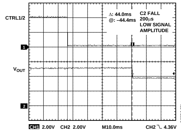
Figure 20. TPC Delay
