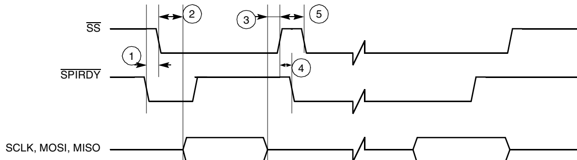
Figure 6. Master CSPI Timing Diagram Using \overline{\text{SPI\_RDY}} Edge Trigger
