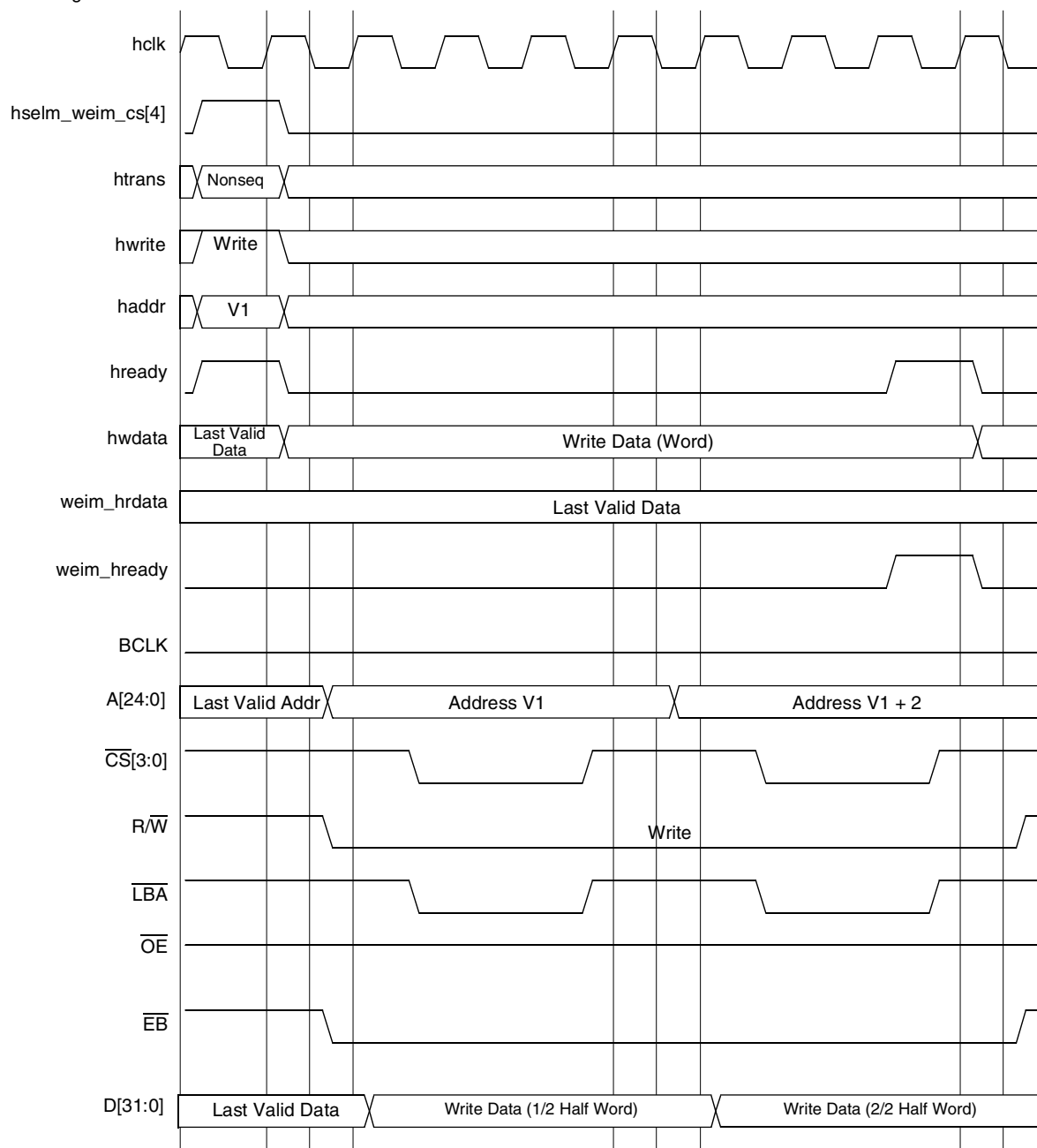
Figure 60. WSC = 2, CSA = 1, WWS = 1, A.WORD/E.HALF
