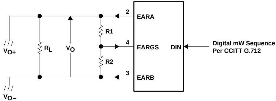
Figure 6. Gain-Setting Configuration
