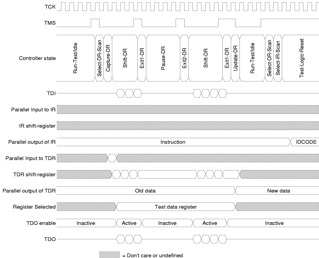
Figure 14. JTAG Data Register update
