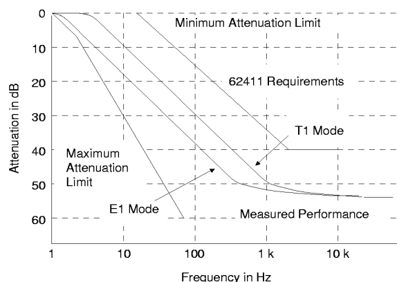
Figure 5. Typical Jitter Transfer Function
