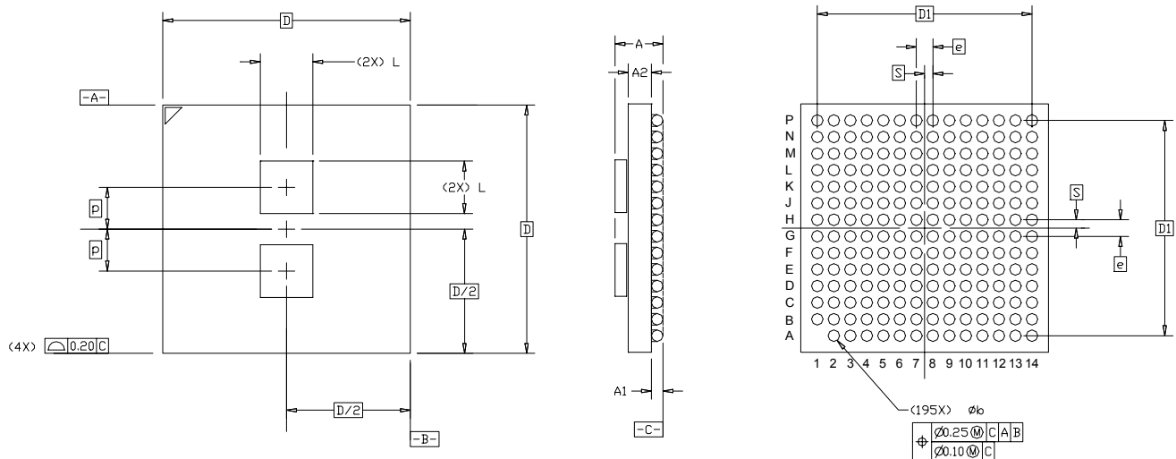
Figure 15. 195-Ball Grid Array (BGA)
