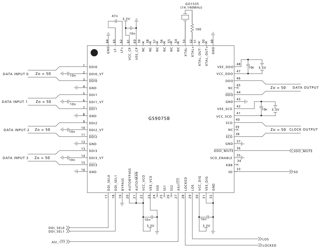
Figure 5-2: GS9075B Typical Application Circuit
