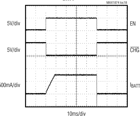
DC STARTUP WAVEFORMS FOR ENABLE V_BATT = 3.9V
