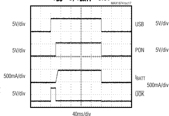
USB CONNECT WAVEFORMS V_DC = 0, V_BATT = 3.9V
