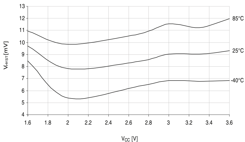
Figure 33-290. Analog comparator hysteresis vs. V_{CC} .
