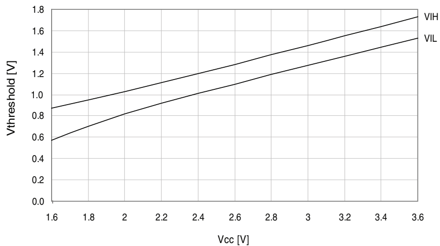
Figure 33-190. I/O pin input threshold voltage vs. V_{CC} .
