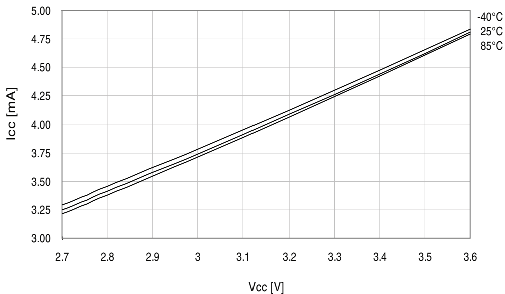
Figure 33-254. Idle mode current vs. V_{CC} .
