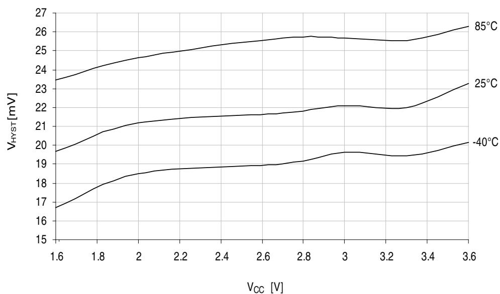
Figure 33-290. Analog comparator hysteresis vs. V_{CC} .
