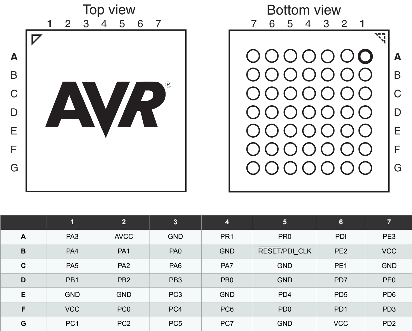
Figure 2-2. VFBGA pinout
