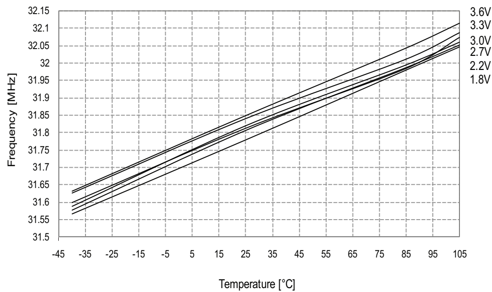
Figure 33-72. 32MHz internal oscillator frequency vs. temperature. DPLL enabled, from the 32.768kHz internal oscillator.
