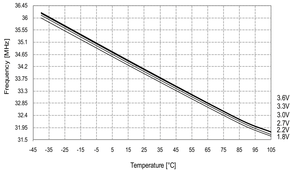
Figure 33-71. 32MHz internal oscillator frequency vs. temperature. DPLL disabled.
