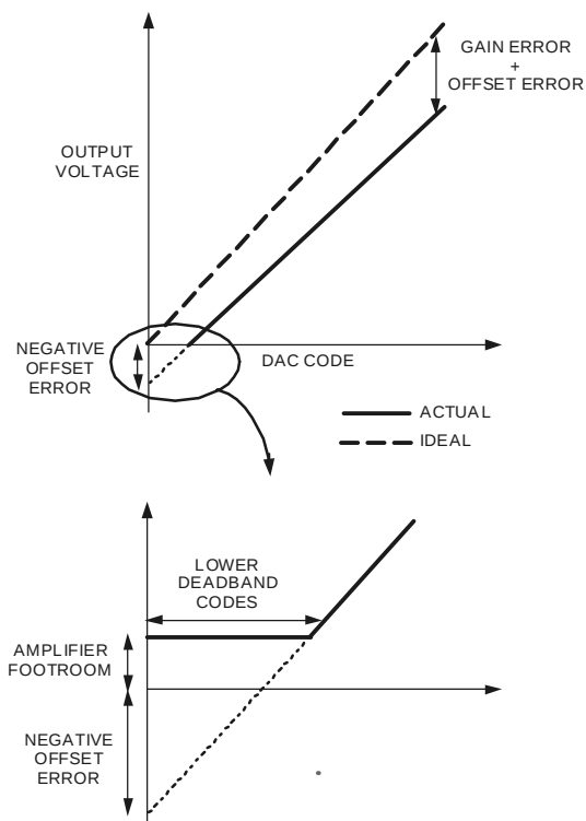
Figure 5. Transfer Function with Negative Offset
