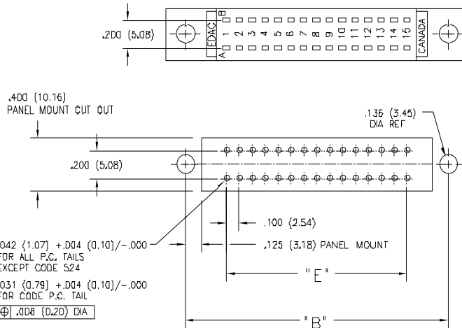
CONNECTOR MOUNTING PATTERN
