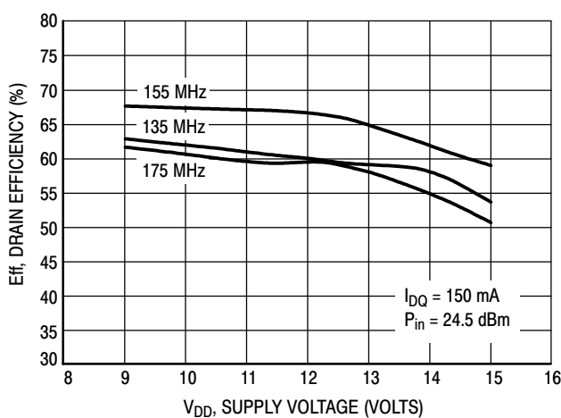
Figure 36. Drain Efficiency versus Supply Voltage
