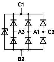
Fig 16. IP4059CX5 Schematic view and package drawing
