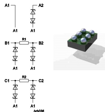
Fig 13. IP4078CX6 Schematic view and device package drawing
