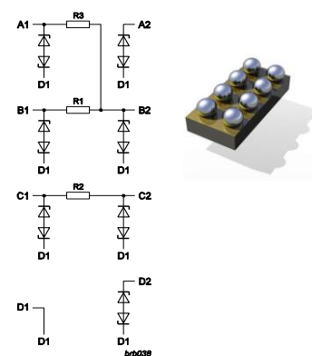
Fig 14. IP4058CX8, IP4158CX8 Schematic view and package drawing
