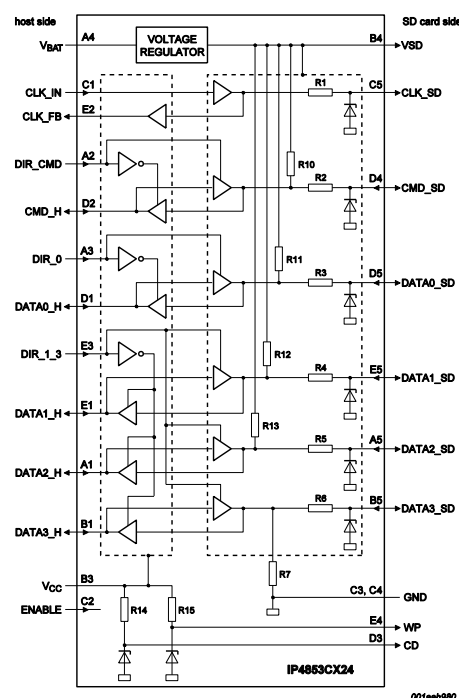
Fig 11. IP4853CX24 schematic
