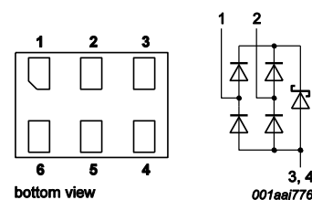
Fig 24. IP4282CZ6 pinning and schematic view
