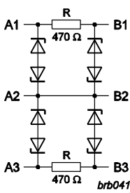
Fig 30. IP4055CX6 & IP4355CX6 Schematic view and depiction of CSP package
