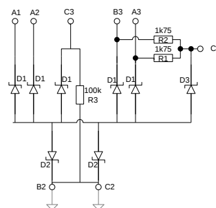
Fig 21. IP4309CX9 schematic view
