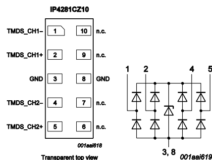
Fig 23. IP428xCZ10 pinning and schematic view
