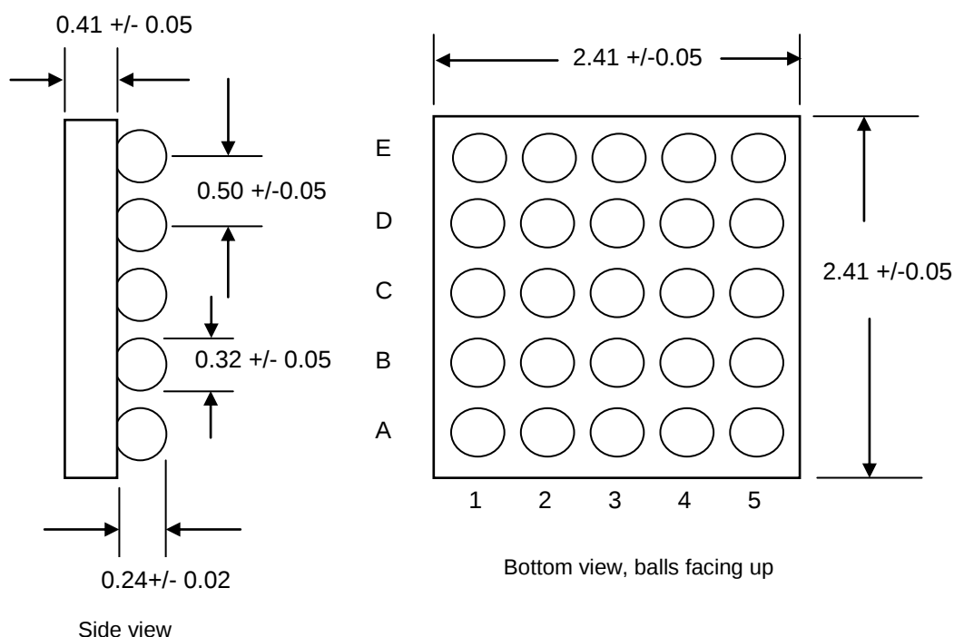
Fig 46. 0.5 mm pitch chip scale package outline
