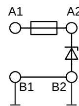
Fig 43. IP4389CX4 schematic view
