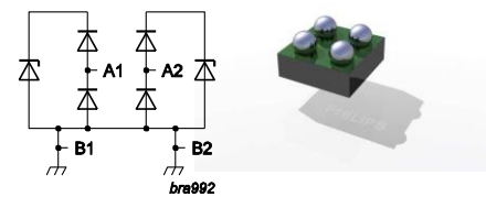
Fig 17. IP4359CX4 Schematic view and package drawing
