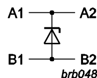
Fig 42. Schematic view of IP4085CX4 & IP4385,6,7CX4
