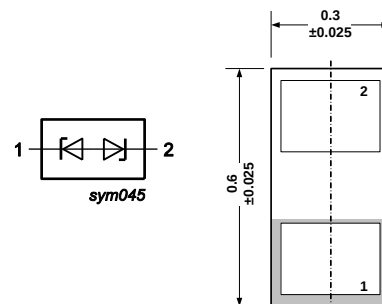
Fig 26. PESD5V0F1BSF schematic symbol and package outline view
