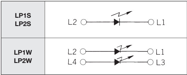
LED Circuit
