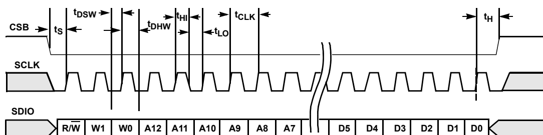
SPI WRITE
