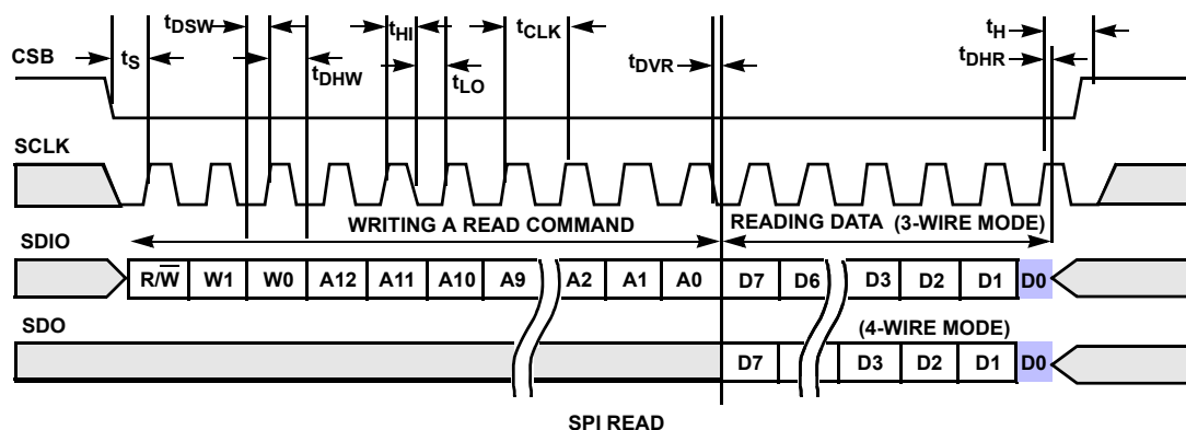
FIGURE 37. SPI READ
