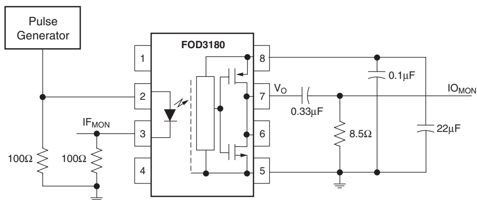
Figure 15. Test Schematic
