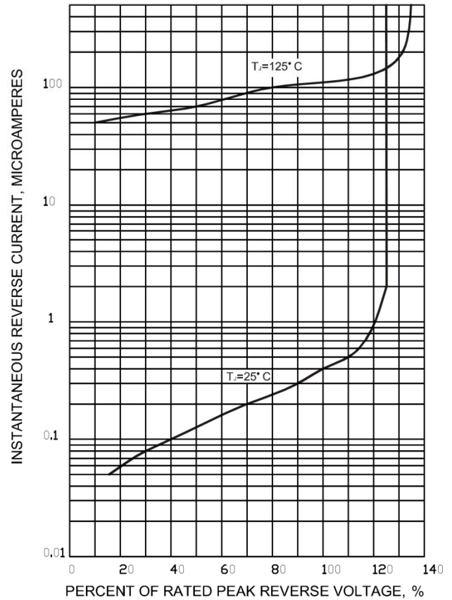
FIG.6-TYPICAL REVERSE CHARACTERISTICS
