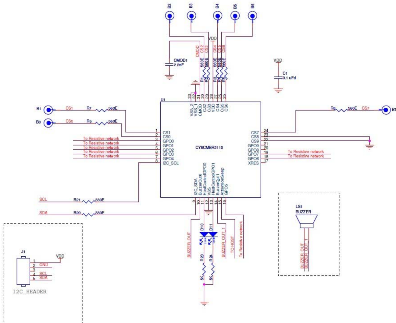
Figure 2. CY8CMBR2110 Schematic 2
