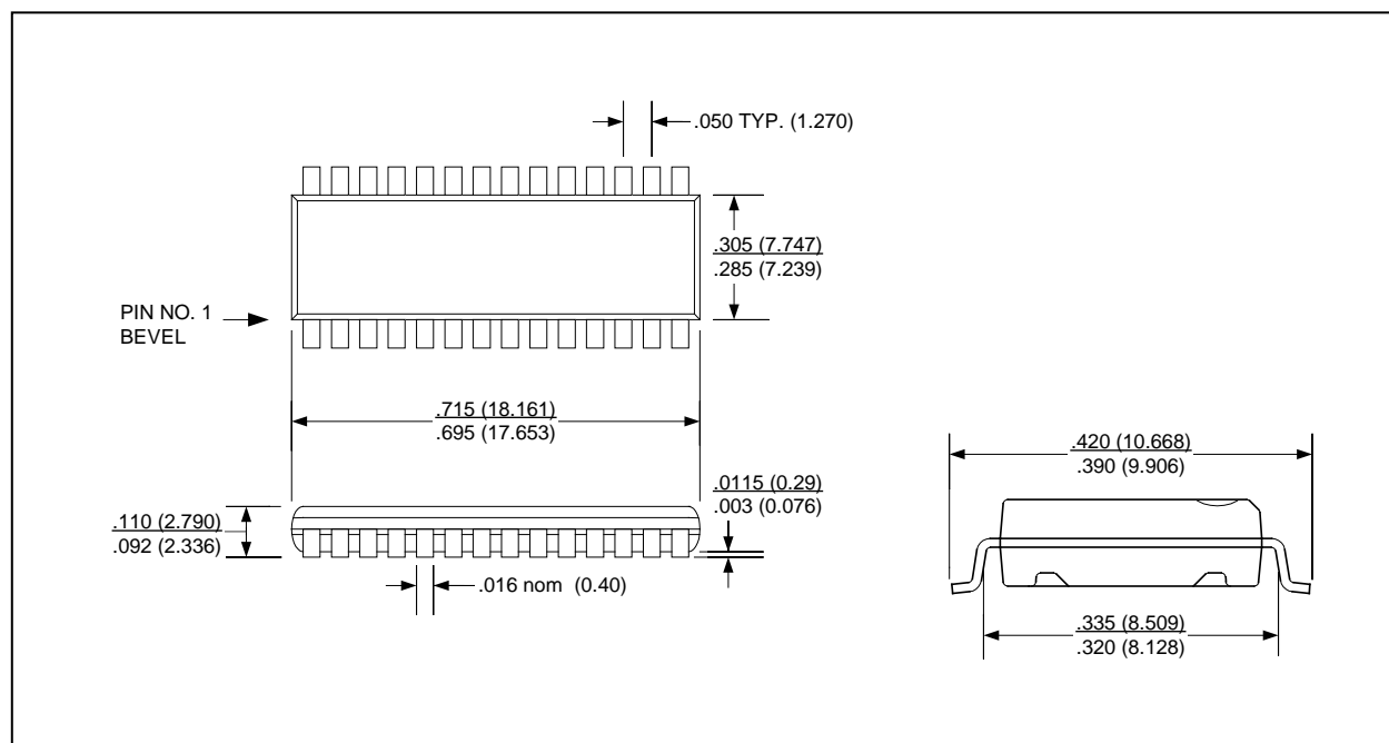
Figure 12: 28 Lead SO
