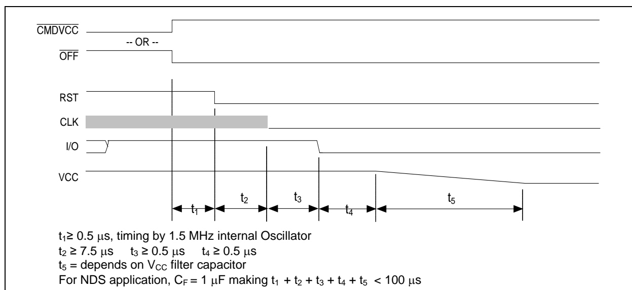
Figure 5: Deactivation Sequence
