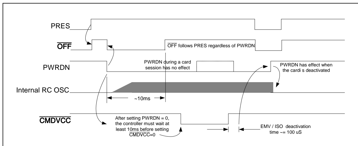
Figure 2: Power Down Mode Operation
