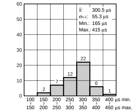
15-(2). Distribution of M.B.B. time Tested sample: TXD2-2M-5V, 50 pcs. Terminal No. 8-9-10: ON
