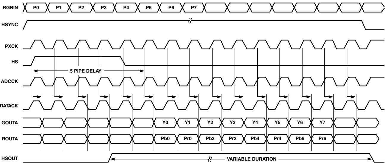
Figure 9. 4:2:2 Mode (for YPbPr Only)
