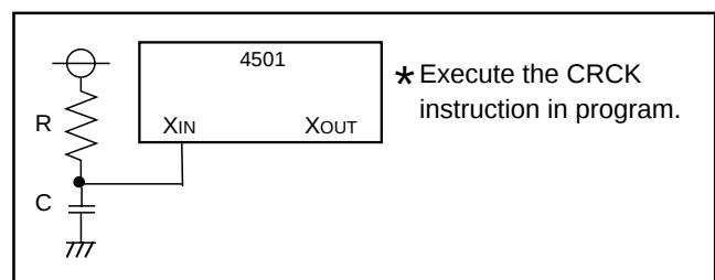
Fig. 45 External RC oscillation circuit
