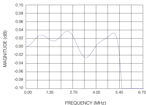
Fig. 4 Frequency Response of Luminance Interpolation Filter (Sampling at f_s=27\text{MHz} )
