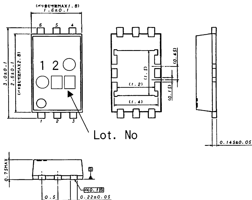
Fig.1 HV S O F 6 (Plastic mold)
