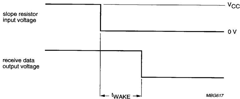
Fig.6 Timing diagram for wake up from standby.
