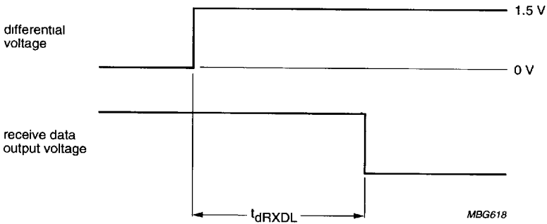
Fig.7 Timing diagram for bus dominant to RXD low.
