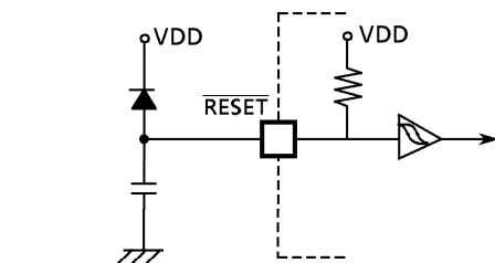
Figure 2-29. Simplified power-on-reset circuit
