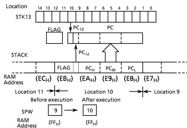
(c) At execution of a subroutine return
