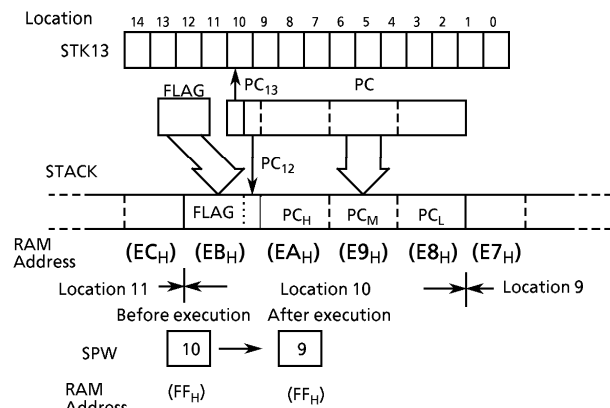
(b) At acceptance of an interrupt instruction
