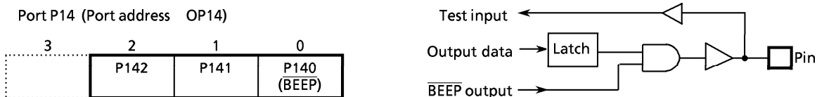
Figure 3-9. Port P14
