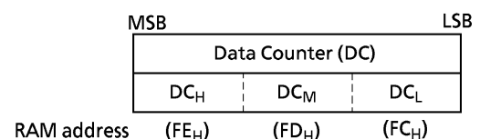
Figure 2-8. Data Counter
