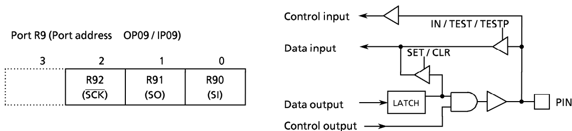
Figure 3-8. Port R9
