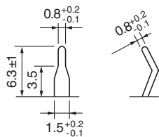
(Terminal dimensions)
