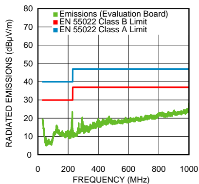
Figure 3. Radiated EMI (CISPR22) V_{IN} = 5.0V , V_{OUT} = 1.8V , I_{OUT} = 1A
