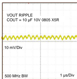
Figure 2. Output Voltage Ripple V_{IN} = 5.0V , V_{OUT} = 1.8V , I_{OUT} = 1A
