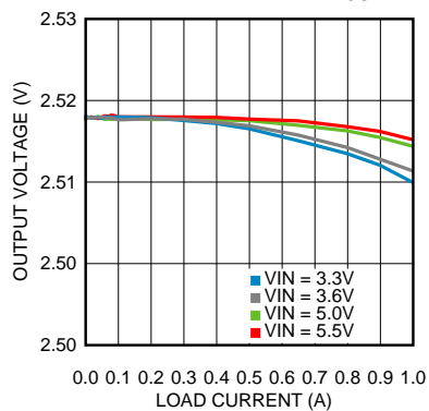
Line and Load Regulation V_{OUT} = 2.5V
