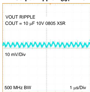
Output Ripple V_{OUT} = 2.5V
