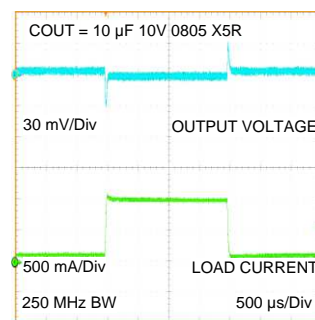
Load Transient V_{OUT} = 2.5V
