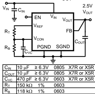
Schematic V_{OUT} = 2.5V
