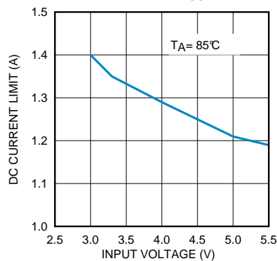
DC Current Limit V_{OUT} = 2.5V
