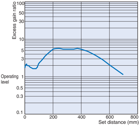
E3T-SR3□ + E39-R37 (Provided)
