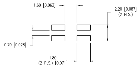
D/C RECOMMENDED SOLDER PAD LAYOUT
