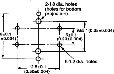
PCB mounting (top view)
