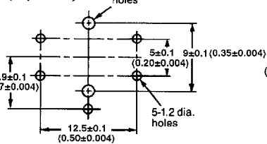
PCB mounting (top view)
